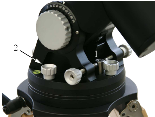
Fig. 4.10: Mount on base adapter.
