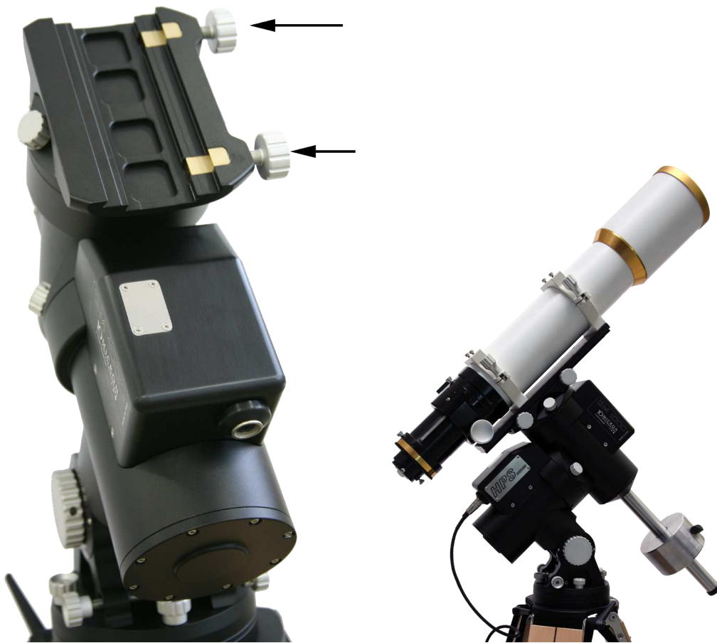
Fig. 4.14: Safety position. Note the position of the dovetail locking knobs on the right of the mount (marked by arrows).
