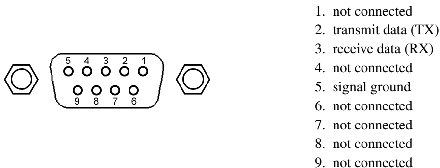
Fig. 5.2: RS-232 port pinout.
