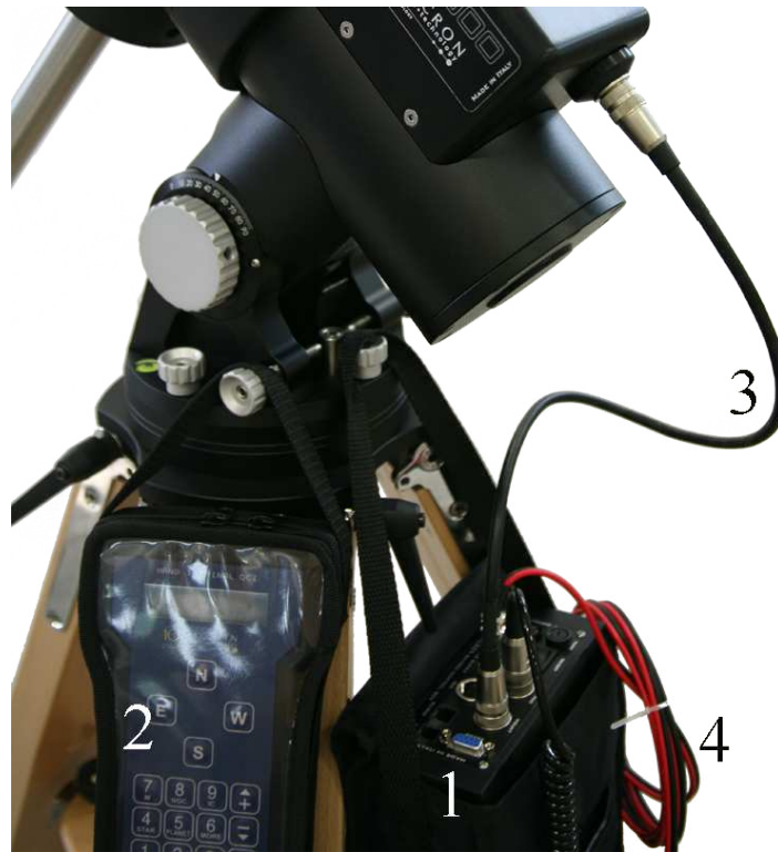
Fig. 5.8: Electrical setup. 1 – control box; 2 – keypad; 3 – mount cable; 4 – power supply cable.
