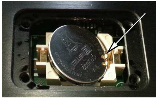
Fig. 5.10: Clock battery replacement.
