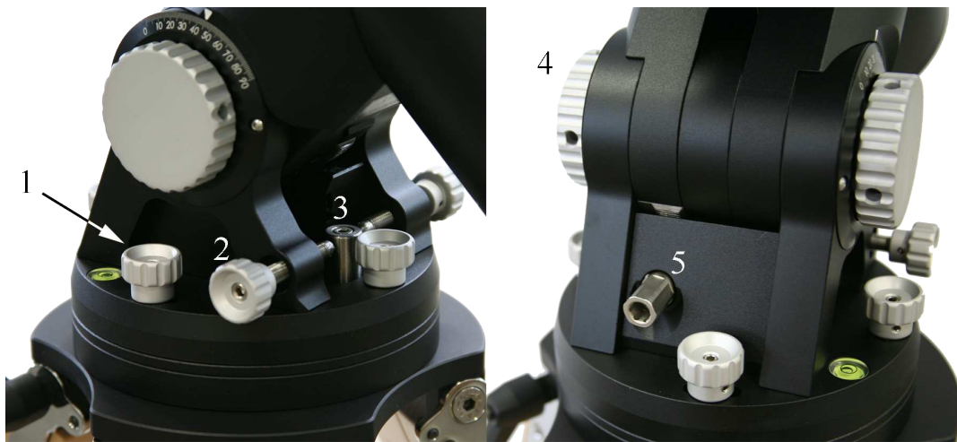
Fig. 4.20: Fine altitude and azimuth adjustment system.
