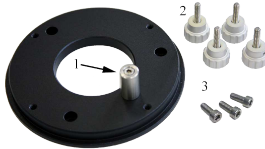
Fig. 4.6: Base adapter assembly and mount locking knobs.
