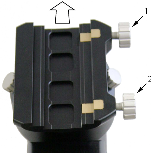
Fig. 4.18: The double-sized dovetail.
