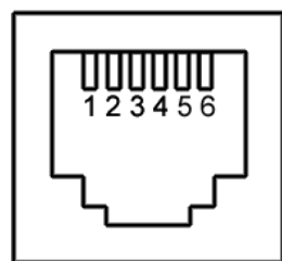
Fig. 5.6: Autoguider port pinout.
