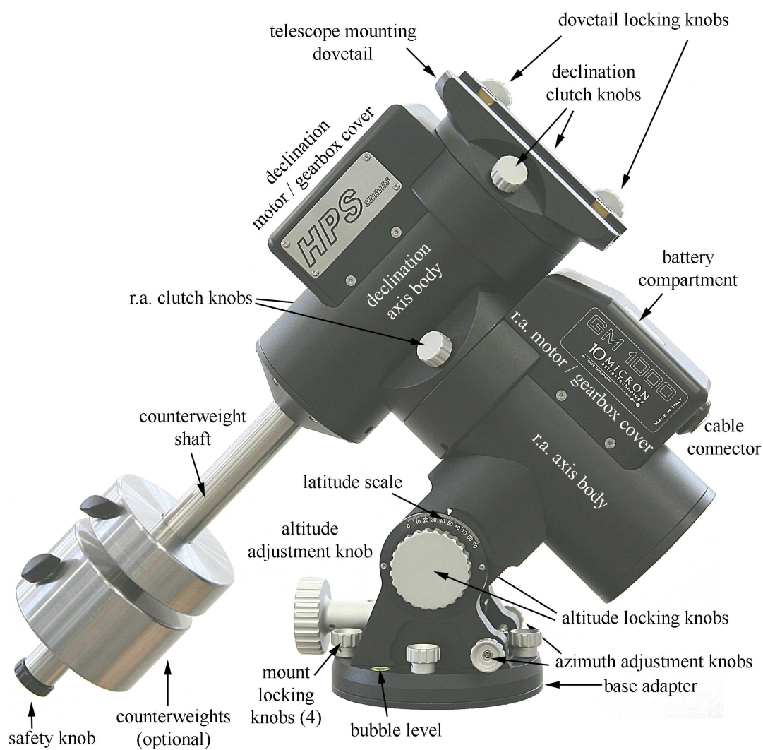
Fig. 4.5: GM1000HPS mount parts.
