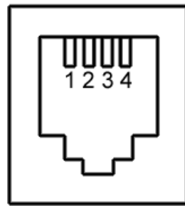
Fig. 5.4: GPS port pinout.
