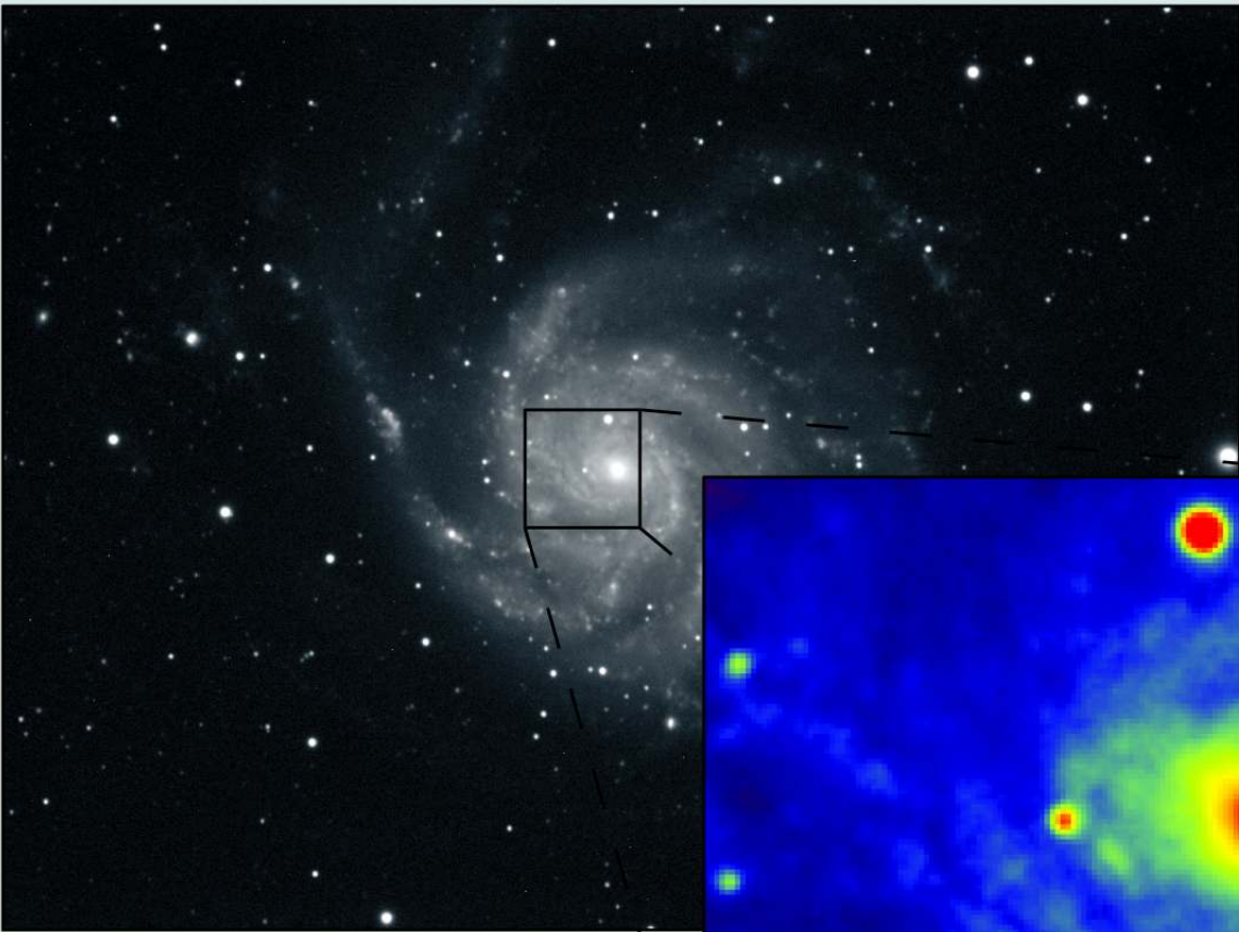
M101. Unguided exposure of 1800s, scale of 1.38"/pixel. Detail in false colors.
