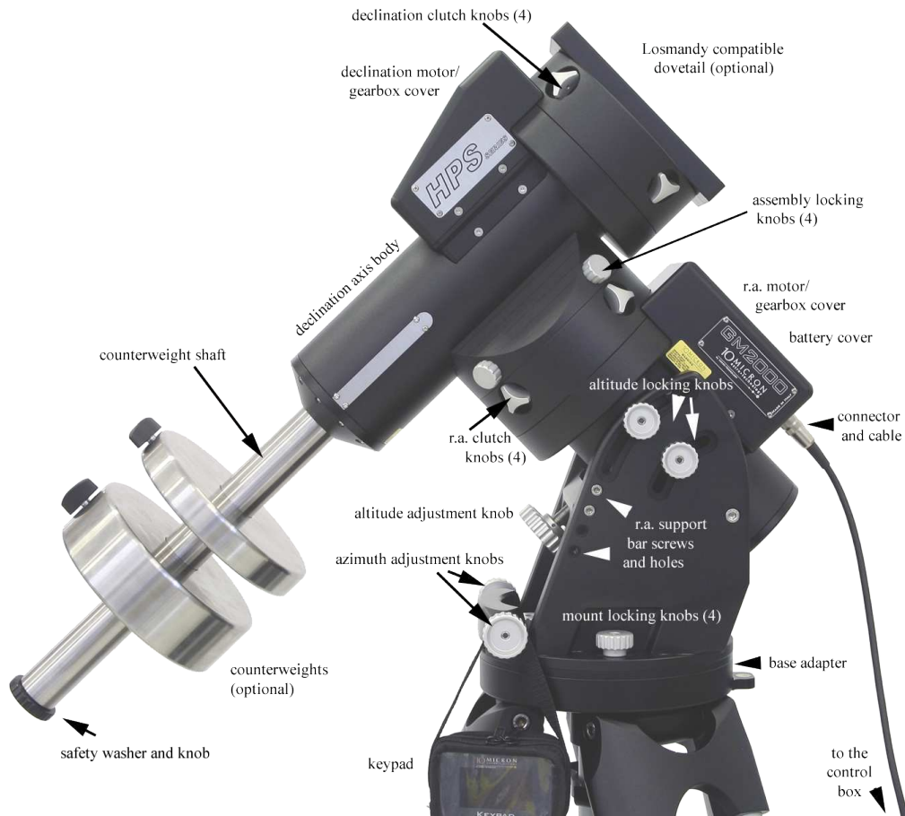
Fig. 4.5: GM2000HPS II mount parts.
